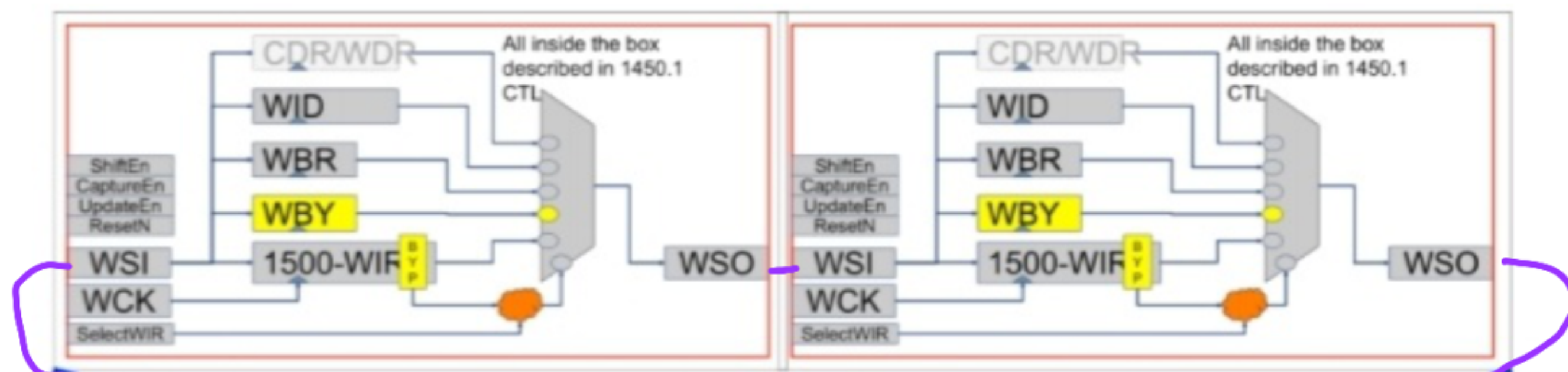
Daisy-Chained 1500 Wrappers
